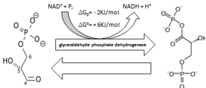
Figure 5: Conversion of D-glyceraldehyde 3-phosphate (GADP) into into 1, 3-bisphosphoglycerate.
